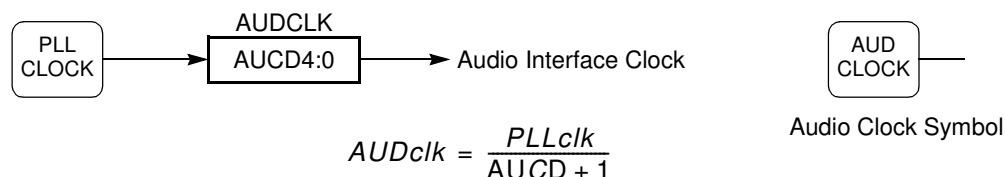
Figure 14. Audio Clock Generator and Symbol
