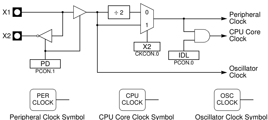
Figure 5. Crystal Connection
