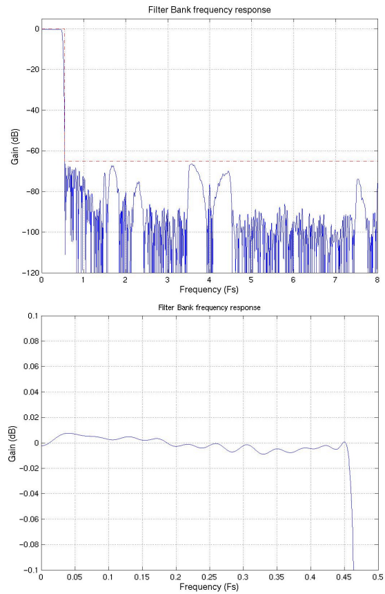
Figure 86. Channel Filter
