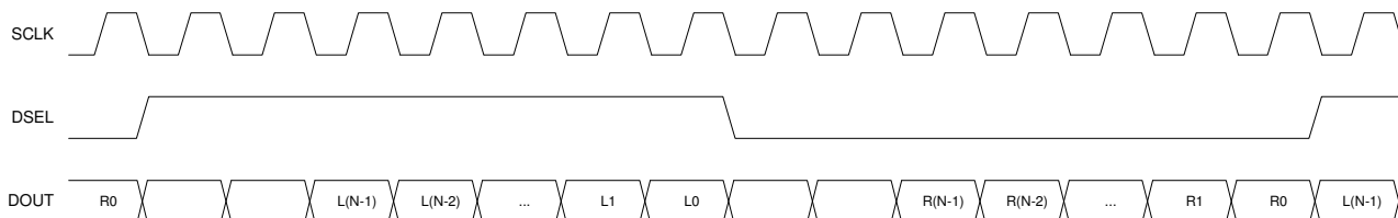
Figure 23. 20 bit LSB justified mode
